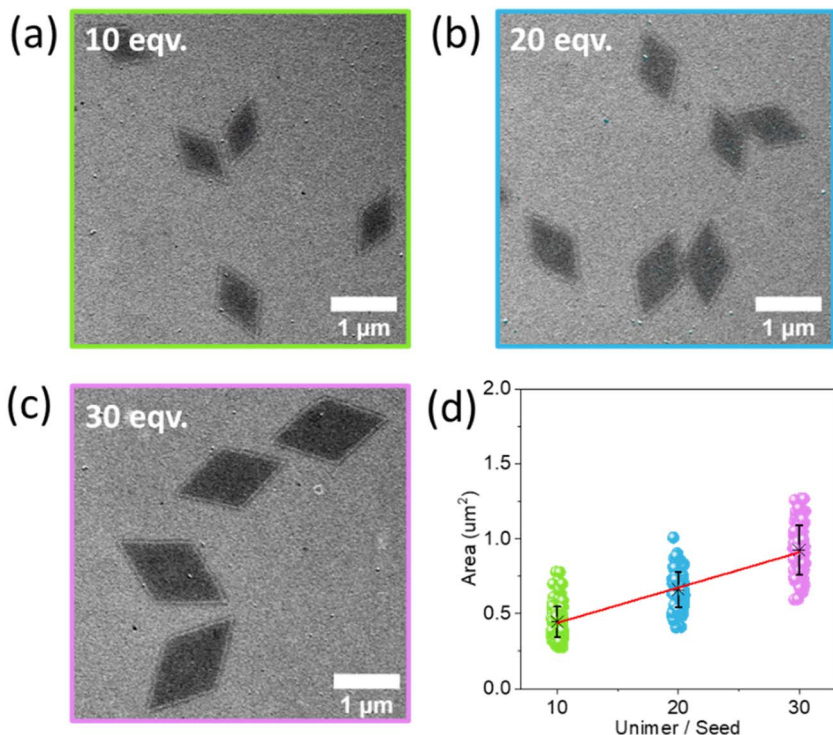
Fig. 4 Size-controllable platelets prepared by living CDSA using PLLA 12 /PLLA 45 - b -PDMAEMA 183 at mass ratio of 1/1: (a), (b), and (c) are TEM images of platelets prepared at various unimer-to-seed ratios, and (d) linear fit of area upon different unimer-to-seed ratios. Scale bar = 1 μm. Platelet size was analyzed from at least 100 particles.
