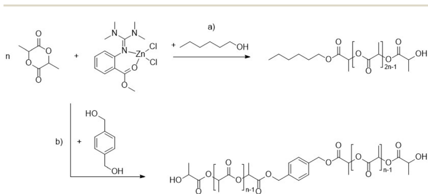
Scheme 1 Lactide ROP catalysed by [\text{ZnCl}_2(\text{TMGasme})] ( C1 ) with two different co-initiators: (a) 1-hexanol ( CoI1 ); (b) 1,4-benzenedimethanol ( CoI2 ).
