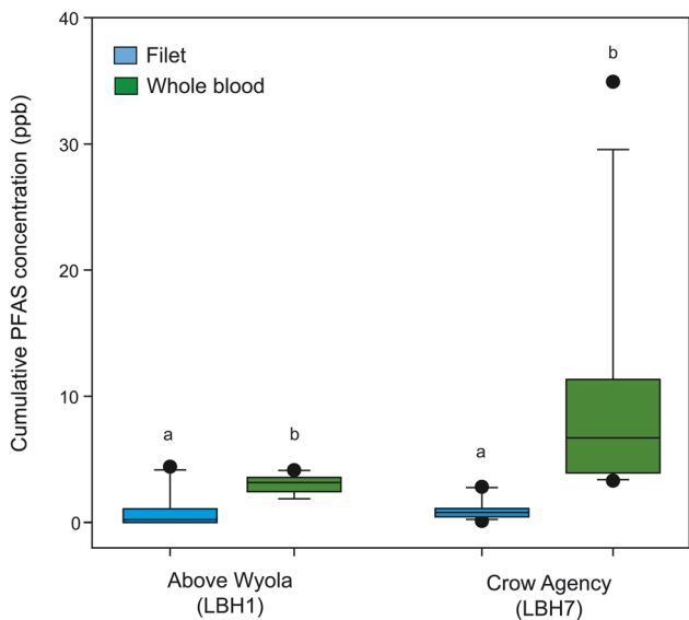
Fig. 5 Cumulative per- and polyfluoroalkyl substances (PFAS) concentrations (ppb) in fish filet ( \text{ng g}^{-1} wet weight) and whole blood ( \text{ng mL}^{-1} ) samples collected from two sites along the Little Bighorn River within the Crow Reservation, Montana. Boxes, centerlines, and whiskers indicate interquartile range, median, and 5th and 95th percentiles, respectively. The letter above boxplot pair indicates the permuted probability that the centroids and dispersions are the same (PERMANOVA; 9999 permutations).
