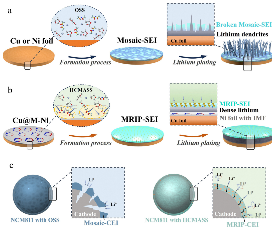
Fig. 1 Magnetized nickel-layer-induced HMASS facilitating uniform lithium deposition. Schematic of lithium plating behavior on (a) Cu or Ni foil and (b) M–Ni coating. (c) Insertion and extraction behaviors of lithium ions in NCM811 with or without M–Ni coating.
