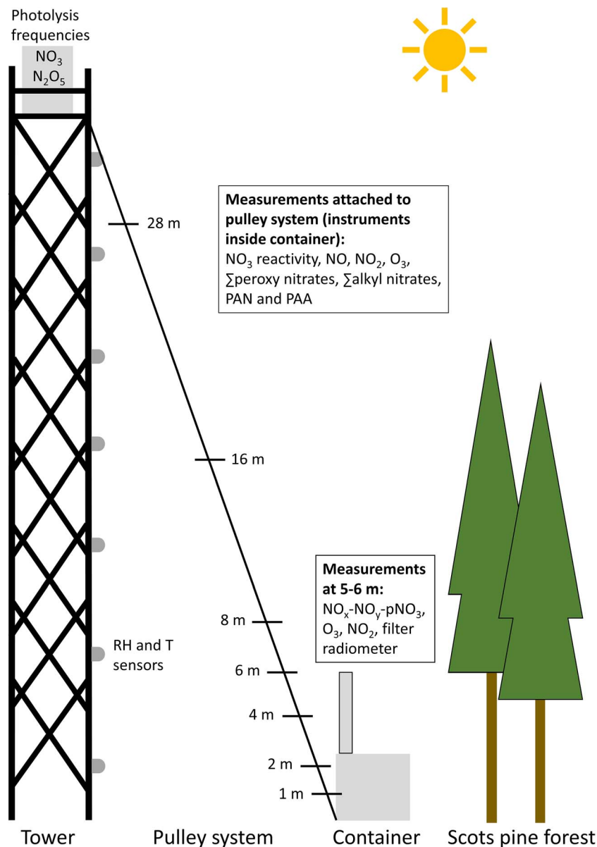
Fig. 1 Schematic showing the instrument and inlet locations during BAIRN-VIP. The inlet heights were 1, 2, 4, 8, 16 and 28 m. The approximate, average tree-top height was ~20–22 m. The stationary, temperature and relative humidity (RH) sensors were at heights of 2, 7, 12, 17, 22, 27 and 32 m agl.
