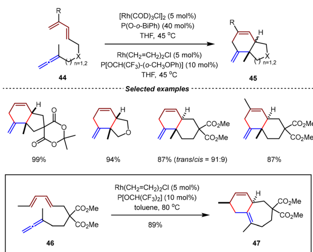
Scheme 14 Rh(I)/phosphite-catalyzed intramolecular [4+2] cycloaddition of 1,1-disubstituted allene-1,3-dienes.
