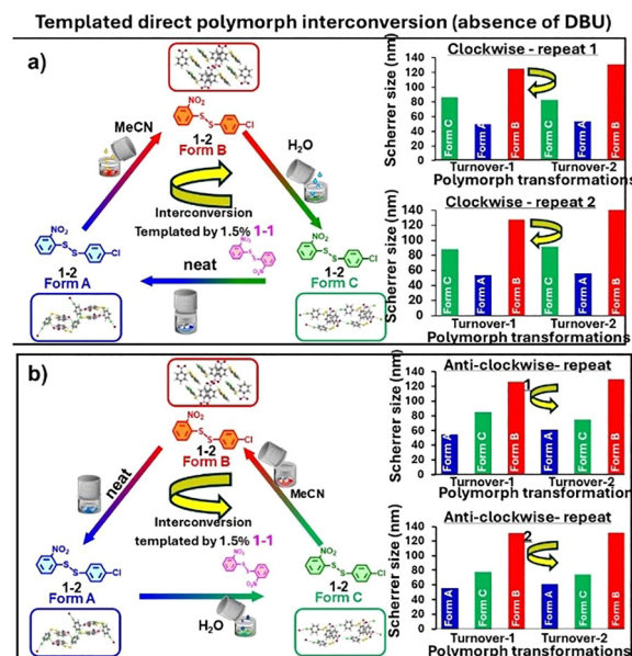
Fig. 35 Three-polymorph interconversion of 1-2 under ball milling. \geq 1.5 mol% 1-1 enables transformations, likely acting as a template. (a) Clockwise: Form B → Form C → Form A → Form B → Form C → Form A → Form B. (b) Anticlockwise: Form B → Form A → Form C → Form B → Form A → Form C → Form B. Form A forms by NG; Form C by LAG with water; Form B by LAG with MeCN. Crystallite sizes: Form A = 40–60 nm; Form C = 70–90 nm; Form B = 120–140 nm. 60 Adapted from ref. 60 with permission from The Royal Society of Chemistry.
