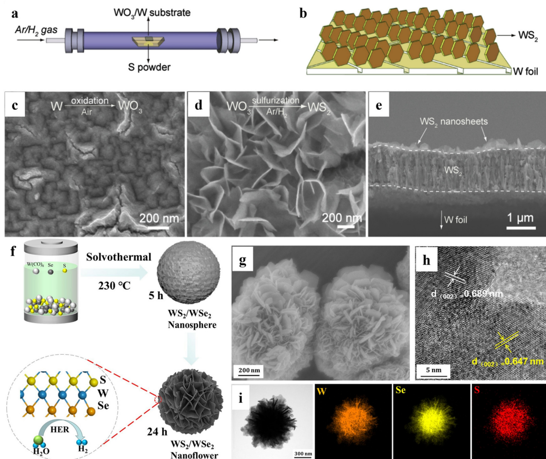
Fig. 3 (a) Schematic illustrating WS_2 synthesis process. (b) Structural diagram of WS_2/W . Scanning electron microscope (SEM) image of (c) WO_3 and (d) WS_2 nanosheets on W foil. (e) Side-view SEM image of WS_2/W . Reprinted with permission. 62 Copyright 2019, Elsevier. (f) Schematic illustration of the synthesis of the flower-like WS_2/WSe_2 heterostructure, (g) SEM image, (h) high resolution transmission electron microscope (HRTEM) image, and (i) high-angle annular dark-field scanning transmission electron microscope (HAADF-STEM) image of flower-like WS_2/WSe_2 heterostructure and energy dispersive X-ray spectroscopy (EDX) elemental mappings image. Reprinted with permission. 64 Copyright 2022, Elsevier.
