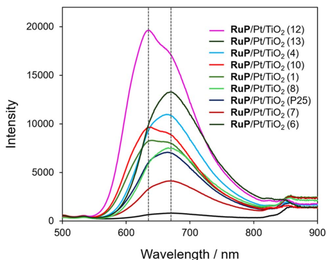
Fig. 5 Emission spectra of RuP/Pt/TiO 2 . Samples were prepared by introducing 3 mg of RuP/Pt/TiO 2 and 4 mL of aqueous HCl solution (pH 4) into a dedicated measurement cell, followed by 30 minutes of Ar bubbling to remove dissolved gases, using an excitation wavelength of 451 nm.
