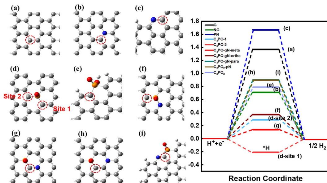
Fig. 7 \Delta G_{\text{H}^*} of (a) graphene (G), (b) graphitic N (NG), (c) pyridinic N (PN), (d) graphene doped with \text{C}_3\text{PO} , (e) graphene doped with \text{C}_2\text{PO}_2 , (f) graphene doped with \text{C}_3\text{PO} and graphitic N in the ortho site ( \text{C}_3\text{PO-gN-ortho} ), (g) graphene doped with \text{C}_3\text{PO} and graphitic N in the meta site ( \text{C}_3\text{PO-gN-meta} ), (h) graphene doped with \text{C}_3\text{PO} and graphitic N in the para site ( \text{C}_3\text{PO-gN-para} ), (i) graphene doped with \text{C}_2\text{PO}_2 and graphitic N ( \text{C}_2\text{PO-pN} ).
