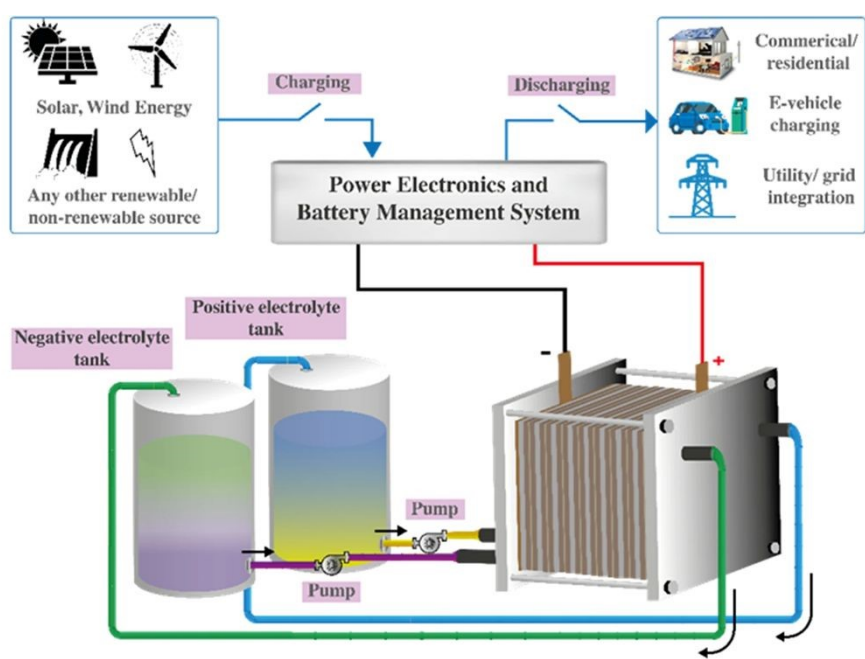
Fig. 1. VFB energy storage schematic 15 (Reprinted with permission of Spinger Nature)
