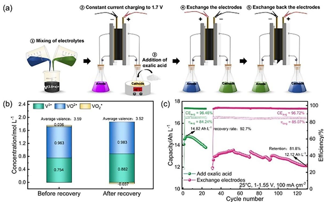
13 Fig. 22 (a) Schematic diagram; (b) Comparison of electrolyte composition; (c)D 14 ischarge specific capacity 112 15
