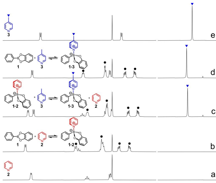
Fig. 4 An exchange experiment in which pyridine 2 (red) and 4-methyl pyridine 3 (blue) compete for phenylboronic acid catechol ester 1 ( \text{CDCl}_3 , 25 °C). All the equilibria are fast on ^1\text{H} -NMR time scale with adduct 1•3 prevailing on adduct 1•2 under competitive conditions (trace c). Trace a 12.5 mM 2 , trace b 12.5 mM 1 and 2 , trace c 12.5 mM 1 , 2 and 3 , trace d 12.5 mM 1 and 3 , trace e 12.5 mM 3 . The black circles are relative to the signals on the 1 backbone.
