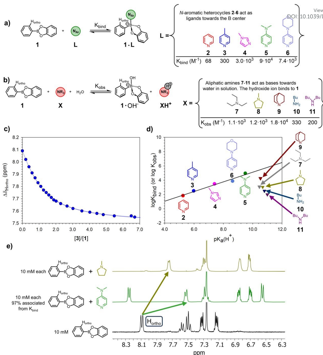
Fig. 1 a) Binding processes between phenylboronic acid catechol ester 1 and N ArHets 2-6 . b) Overall proposed transformation occurring in the presence of amines 7-11 . c) 1 H-NMR titration of 5.0 mM 1 with 3 in CDCl 3 at 25 °C (see ESI, Figures S23-S32 for the other titrations). d) Brønsted correlation between log K bind (or log K obs , for aliphatic amines 7-11 ) and p K a H + for compounds 2-11 (for pyridines, p = 0.68, R 2 = 0.97, see ESI, Table S2 for details). The linear correlation only holds for N ArHets 2-6 ; the data points relative to amines 7-11 lay outside the line. e) Comparison of 1 H-NMR traces of 1 (bottom, black), a mixture of 1 and 5 (centre, green), and a mixture of 1 and 8 (top, gold). Spectra recorded at 25 °C; all compounds are 10 mM in CDCl 3 . Only the aromatics portion is shown. See Figures S51 for full spectra. The H ortho protons on the phenyl moiety on 1 are rendered equivalent in the 1 H-NMR spectra by the fast rotation about the Ph–B bond.
