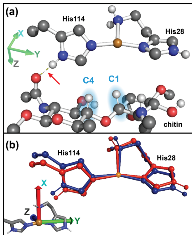
Fig. 11 (a) Optimized structure for Cu(I) SmAA10A ·chitin indicating the hydrogen-bonding interaction (red arrow) between N_{\text{His114}}^{61} and an acetamidyl O from chitin. (b) Overlay of Cu(I)- SmAA10A (blue) and Cu(I)- SmAA10A ·chitin (red) depicting the change induced in His114 upon chitin binding. The Cu site is depicted in orange.
