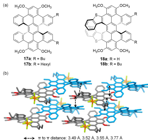
Fig. 6 (a) Double helicenes 17a/b and 18a/b; (b) \pi – \pi stacking in the crystal of 17a^{+\bullet}PF_6^- , where the (M, M) enantiomer is shown in blue, and the (P, P) enantiomer is colored according to the elements. Reproduced with permission from ref. 40. Copyright 2022 American Chemical Society.
