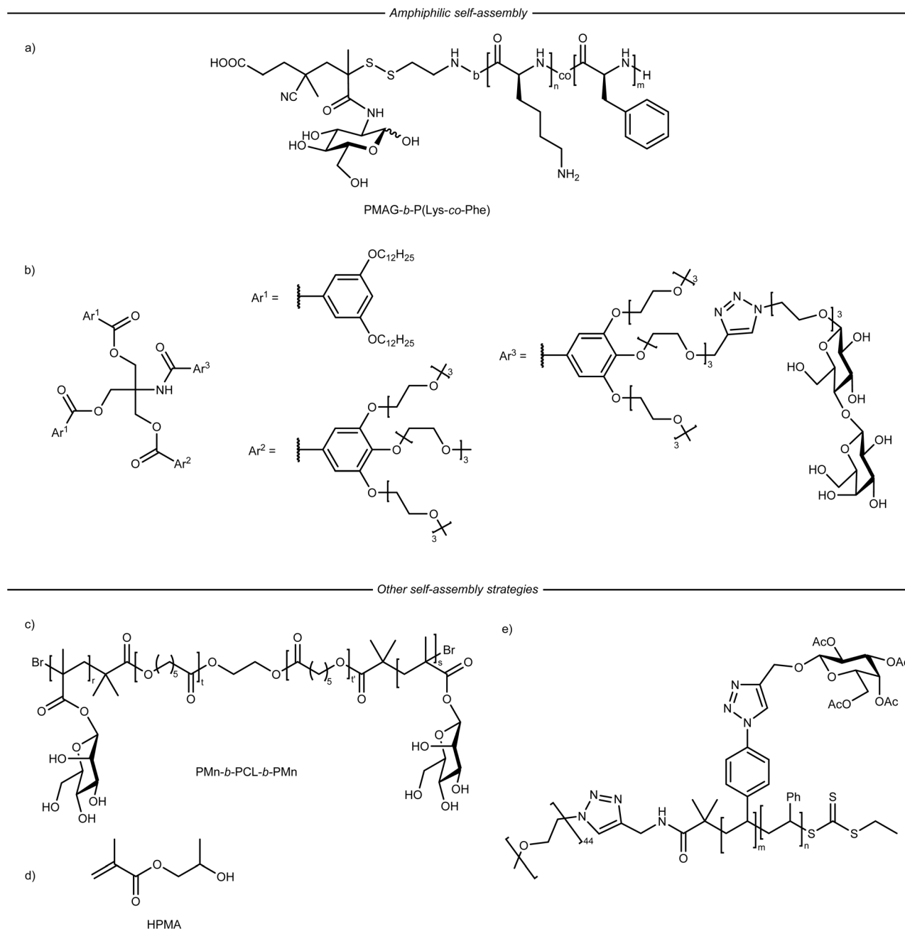
Fig. 4 Representative glycopolymer structures employed in the formation of glycopolymer-based nanoplatoms via self-assembly. (a) Structure of amphiphilic PMAG- b -P(Lys-co-Phe) copolymer forming spherical glycopolymer-based nanoplatoms; (b) structure of amphiphilic Janus glycodendrimers bearing sequence-defined oligomannose for the formation of glycodendrimersomes; (c) structure of mannose-mimicking ABA-type triblock copolymer (PMn- b -PCL- b -PMn), which electrostatically co-assembles with dihexadecyldimethylammonium bromide (DHDAB); (d) structure of hydroxypropyl methacrylate (HPMA) grafted onto dextran backbone, enabling UV-induced self-assembly into nanostructures; (e) representative glycopolymer structure applied in the "glyco-side" strategy.
