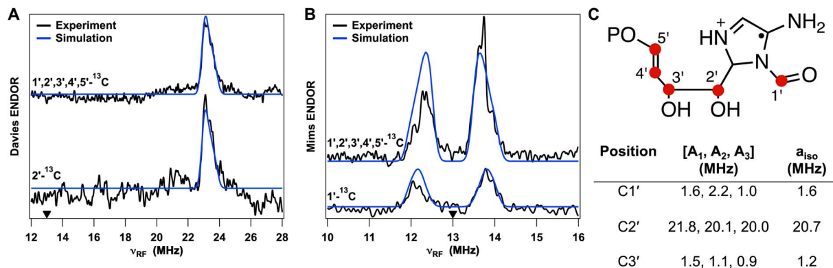
Fig. 4 (A) 13 C Davies ENDOR spectra for the ThiC reaction using 1',2',3',4',5'- 13 C and 2'- 13 C labeled AIR. (B) 13 C Mims ENDOR spectra for the ThiC reaction using 1',2',3',4',5'- 13 C and 1'- 13 C labeled AIR. (C) HFI obtained from spectral simulations with their positions shown for the proposed intermediate 7-H + . Simulations are shown in blue. The 13 C Larmor frequency (13 MHz) is marked by a triangle. Conditions: frequency = 34 GHz, temperature = 15 K. 13 C Davies: \pi/2 = 12 ns, inversion pulse = 80 ns, \tau = 300 ns. 13 C Mims: \tau = 260 ns. Simulations: (A) A 13 C = [21.8, 20.1, 20.0] MHz. (B) Top: A 13 C = [1.6, 2.2, 1.0] MHz, [1.5, 1.1, 0.9] MHz. Bottom: A 13 C = [1.6, 2.2, 1.0] MHz.
