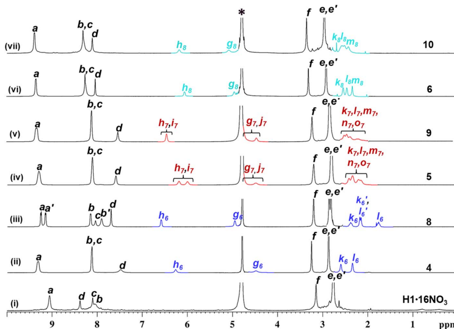
Fig. 6 ^1\text{H} NMR spectra (400 MHz, \text{D}_2\text{O} , 298 K, i.e. , 25 ^\circ\text{C} ) for isolated samples of (i) \text{H1}\cdot 16\text{NO}_3 , (ii) [(\text{H6})_2\subset\text{H1}]\cdot 16\text{NO}_3 (4), (iii) [(\text{G}\subset(\text{H6})_2)\subset\text{H1}]\cdot 17\text{NO}_3 (8), (iv) [(\text{H7})_2\subset\text{H1}]\cdot 16\text{NO}_3 (5), (v) [(\text{G}\subset(\text{H7})_2)\subset\text{H1}]\cdot 17\text{NO}_3 (9), (vi) [(\text{H8})_2\subset\text{H1}]\cdot 16\text{NO}_3 (6), and (vii) [(\text{G}\subset(\text{H8})_2)\subset\text{H1}]\cdot 17\text{NO}_3 (10).
