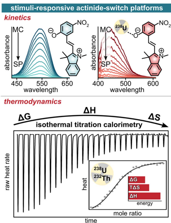
Scheme 1 (Top) photoisomerization kinetics of a stimuli-responsive spiroropyran derivative in the absence (blue) and presence (red) of actinides studied by UV-vis spectroscopy. (Bottom) thermogram obtained through isothermal titration calorimetry used in this work for estimation of Gibbs free energy, enthalpy, and entropy of stimuli-responsive actinide binding.
