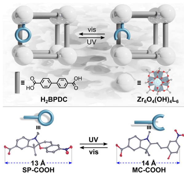
Fig. 2 (Top) schematic representation of spirocyan derivative photoisomerization within a UiO-67 MOF upon exposure to UV or visible light. The structures of the corresponding organic linker (gray rod) and metal node (white sphere) are shown. The blue polyhedra, as well as the gray and red spheres, represent zirconium, carbon, and oxygen atoms, respectively. (Bottom) X-ray crystal structures of SP-COOH and MC-COOH, demonstrating the change in the length of the molecular backbone upon photoisomerization. The gray, red, and blue ellipsoids represent carbon, oxygen, and nitrogen atoms, respectively. Hydrogen atoms have been omitted for clarity. Displacement ellipsoids are drawn at the 80% probability level.
