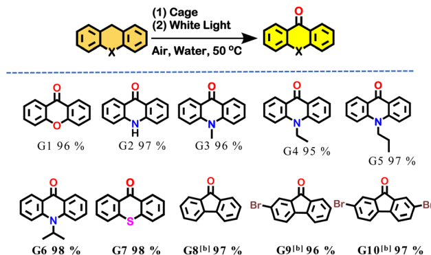
Fig. 6 Scope of the aqueous cage 1 catalyzed C(sp 3 )-H oxidation of alkylarenes. The yield is calculated by ^1\text{H} NMR using 1,3,5-trimethoxybenzene as an internal standard [b: a 390 nm 100 W LED was used]. The % conversion was calculated by ^1\text{H} NMR using the internal standard 1,3,5-trimethoxybenzene.
