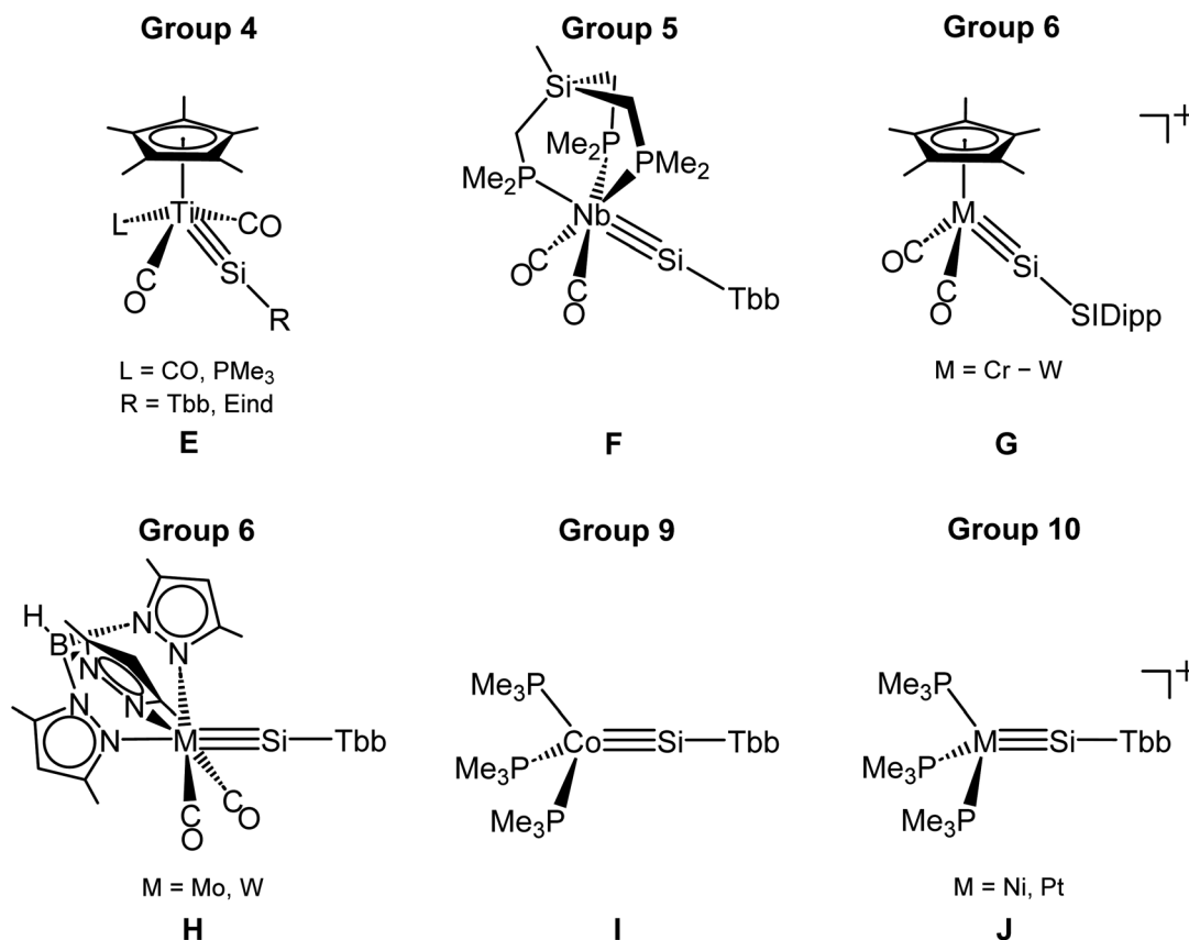
Fig. 2 Silyldiene complexes of various transition metal groups isolated and fully characterized in our group; \text{SIDipp} = \text{C}[\text{N}(\text{Dipp})\text{CH}_2]_2 , \text{Dipp} = 2,6\text{-diisopropylphenyl} ; \text{Tbb} = \text{C}_6\text{H}_2\text{-2,6-(CH(SiMe}_3)_2)_2\text{-4-tBu} ; \text{Eind} = 1,1,3,3,5,5,7,7\text{-Et}_8\text{-s-hydrindacene-4-yl} .
