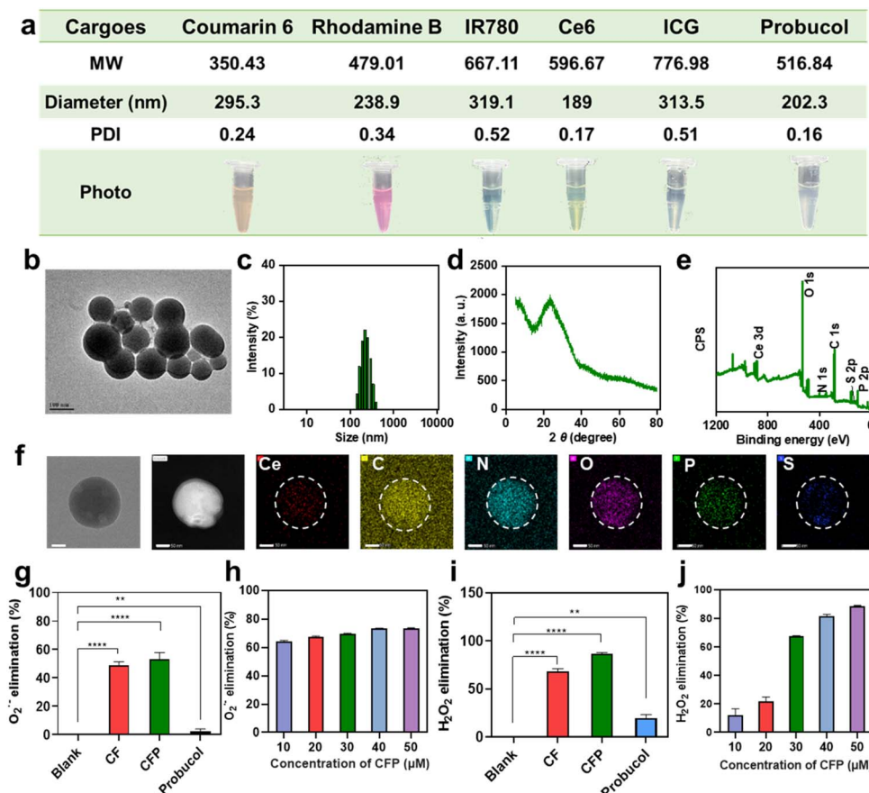
Fig. 2 Moonlighting protein-like multi-functions of CF nanoassembly. (a) CF as a nanocarrier for the loading of different cargoes (Coumarin 6, Rhodamine B, IR780, Ce6, ICG, and probucon). (b) TEM image of CFP, scale bar: 100 nm. (c) Hydrodynamic diameter of CFP. (d) XRD pattern of CFP. (e) XPS survey spectrum of CFP. (f) EDS elemental mapping images of CFP. Scale bar: 50 nm. (g) O_2^{\cdot-} -eliminating capabilities of CF, CFP and probucon. (h) CFP concentration-dependent O_2^{\cdot-} -eliminating capability. CFP concentration is represented as Ce concentration. (i) H_2O_2 -eliminating capabilities of CF, CFP and probucon. (j) CFP concentration-dependent H_2O_2 -eliminating capability. CFP concentration is represented as Ce concentration.
