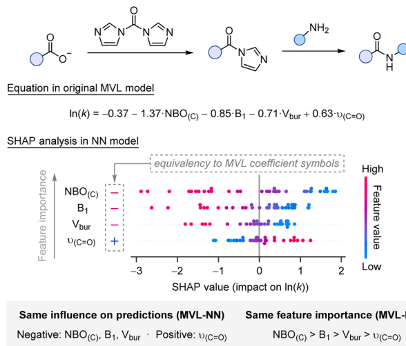
Fig. 5 Comparison of the original MVL equation with the SHAP analysis of the new NN model.
