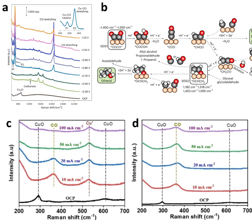
Fig. 6 (a) Raman spectra obtained from electrochemically treated Cu foil during \text{eCO}_2\text{RR} within potentials range from the open-circuit potential (OCP) to about -1.1 V vs. RHE in a 0.1 M \text{NaClO}_4 electrolyte that had been saturated with \text{CO}_2 gas. (b) Proposed reaction scheme for the generation of ethylene and ethanol. (a) and (b) are reproduced from ref. 119 with permission from Springer Nature Link, copyright 2024. Operando Raman spectra analysis during \text{CO}_2\text{RR} at varying current densities. (c) \text{CuO}_x\text{@C} . (d) \text{CuO}_x . (c) and (d) are reproduced from ref. 122 with permission from Wiley, copyright 2022.
