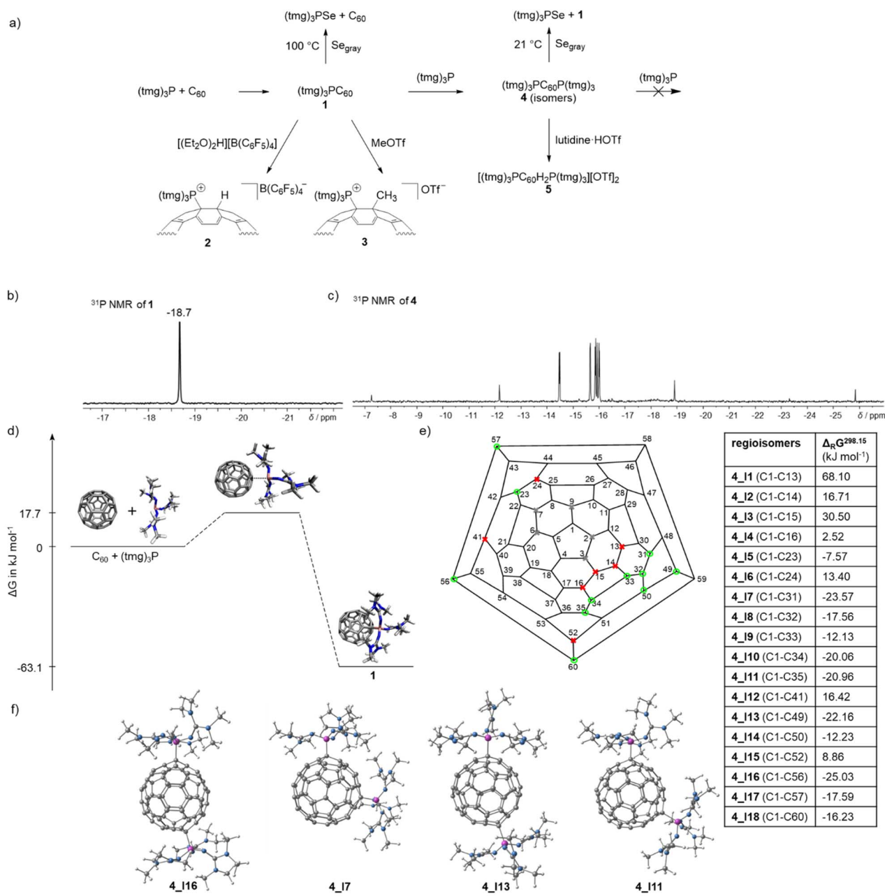
Fig. 4 (a) Overview of the reactivity of 1 and 4 ; (b) 31 P NMR spectrum of the monoadduct 1 in THF; (c) 31 P NMR spectrum in THF of the bisadducts (tmg) 3 PC 60 P(tm g ) 3 ( 4 ) obtained as mixture of positional isomers; (d) reaction energy profile for the formation of 1 determined by DFT using B3LYP(GD3BJ)/6-31G(d,p)/SMD(THF); (e) calculated free energies for the formation of the positional isomers 4 according to: 1 + (tmg) 3 P → 4 determined by DFT using B3LYP(GD3BJ)/6-31G(d,p)/SMD(THF), Schlegel diagram of C 60 with possible structural isomers 39 if one phosphonium center is located at C1 (gray: positional isomers with less than three CC bond between the phosphonium centers that were not considered for steric reasons, red: endergonic isomers, green: exergonic isomers); (f) optimized geometries of the four most stable isomers of 4 .
