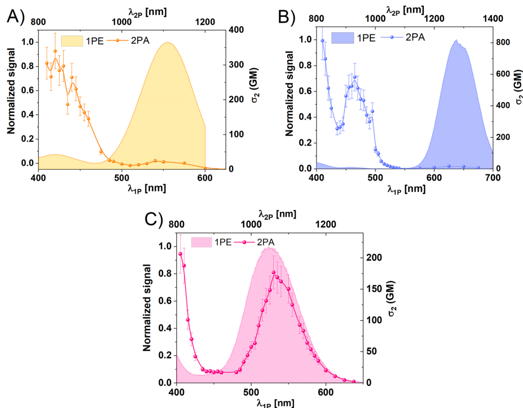
Fig. 2 Comparison between one photon excitation (1PE, filled bands) and two photon absorption (2PA, points and lines) of (A) \text{Ag}_{15} -DNA, (B) \text{Ag}_{21} -DNA, (C) \text{Ag}_{16} -DNA-Cl 2 .
