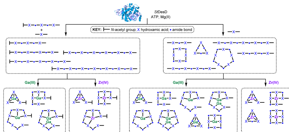
Scheme 4 Biocombinatorial pools of hydroxamic acid chelators (3–14) in cartoon form produced by StDesD-mediated synthesis using as substrates 1 and 2 (left path; compounds contain a terminal amine group) or 2 (right path; linear compounds contain flanking amine and carboxylic acid groups) and coordination complexes characterised in situ upon incubation of each pool with Ga(III) or Zr(IV). The structure of StDesD was produced by AlphaFold. 39
