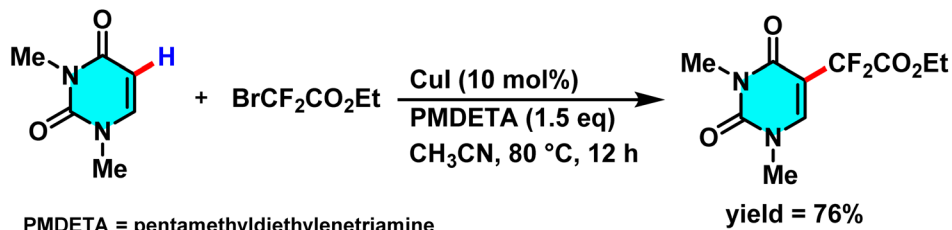
Scheme 28 Cu(I)-catalyzed C–H difluoroalkylation of pyrimidine.
