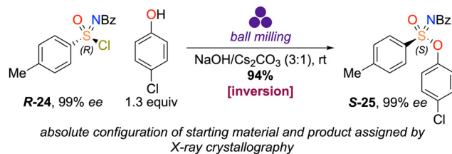
Scheme 6 Mechanochemical synthesis of sulfonylimidate S-25 from sulfonylimidoyl chloride R-24 , with confirmation of sulfur stereocenter inversion by X-ray crystallography.
