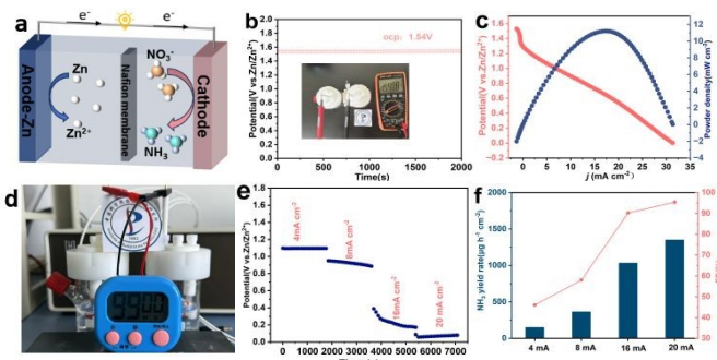
Fig. 6 (a) Schematic illustration of the Zn-NO 3 - battery assembled with the CuO-Fe 3 O 4 /CNTs cathode. (b) OCV curve of the Zn-NO 3 - battery assembled with the CuO-Fe 3 O 4 /CNTs cathode. Inset of (b) shows the photograph of the OCV measurement of the Zn-NO 3 - battery. (c) Discharging curves and the corresponding power density plot. (d) Digital photos of the electronic timer powered by this Zn-NO 3 - battery. (e) Discharging tests at different current densities of this Zn-NO 3 - battery. (f) NH 3 FE and NH 3 yield rates in the discharge process (we assembled a rechargeable Zn-NO 3 - battery using highly active CuO-Fe 3 O 4 /CNTs as the cathode).
