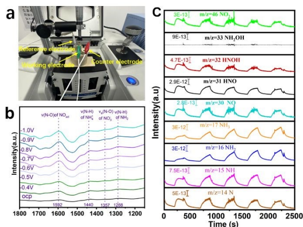
Fig. 5 (a) Physical photograph of in-suit ATR-SEIRAS reactor for (b) In-situ ATR-SEIRAS spectra of electrocatalytic NitRR on CuO-Fe 3 O 4 /CNTs at different potentials in the 0.1 M KOH + 0.1 M KNO 3 electrolyte. (c) In-situ DEMS measurements for CuO-Fe 3 O 4 /CNTs in the 0.1 M KOH + 0.1 M KNO 3 electrolyte at -0.8V (vs. RHE) for the NitRR.
