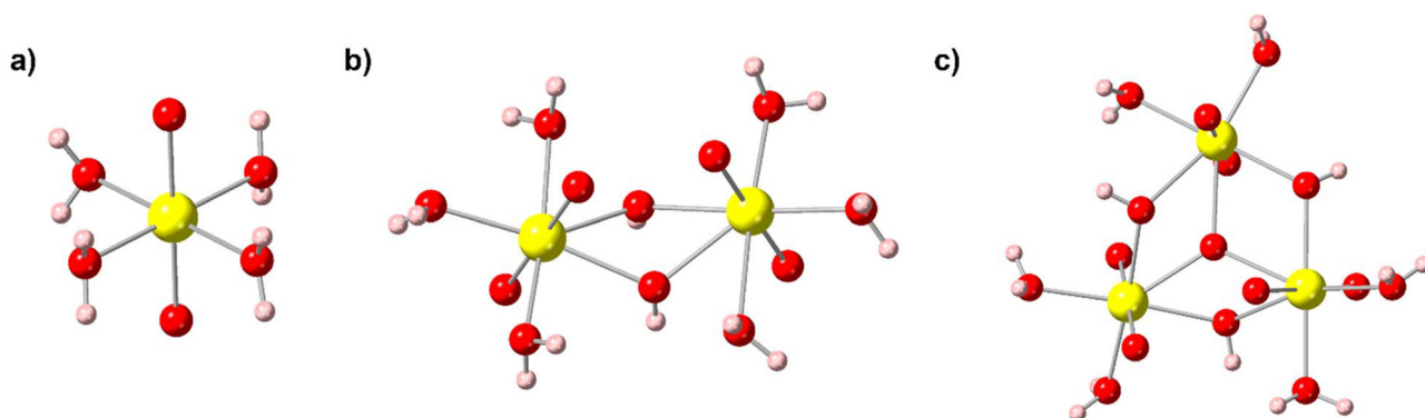
Fig. 7 Uranyl (UO 2 2+ ) complexes that can exist in aqueous solutions with hydroxide anions. (a) [UO 2 (H 2 O) 4 ] 2+ , (b) [UO 2 (OH) 2 (H 2 O) 4 ] 2+ , and (c) [UO 2 (O)(OH) 3 (H 2 O) 4 ] + . U, O, and H are depicted as yellow, red, and pink spheres, respectively. Adapted from Quilès et al. 71
