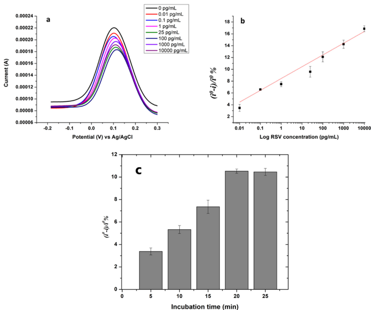
Fig. 3 (a) Square wave voltammograms recorded for the GOx/Mo 2 Ti 2 C 3 T x /SPCE immunosensor towards increasing concentrations of the RSV antigen (0, 0.01, 0.1, 1, 25, 100, 1000 and 10 000 pg mL -1 ) prepared in PBS. (c) Effect of the binding time on the response of the RSV immunosensor. The measurements were carried out in a 5 mM ferri/ferrocyanide solution in PBS buffer at a pH of 7.4. The measurements were recorded in the ferro/ferricyanide electrolyte in the range of -0.2 to 0.3 V, at an interval time of 0.04 s, a frequency of 25 Hz, a scan rate of 125 mV s -1 , an amplitude of 20 mV, and a step potential of -5 mV. (b) Plot of the sensor's response versus the logarithm of RSV antigen concentrations.
