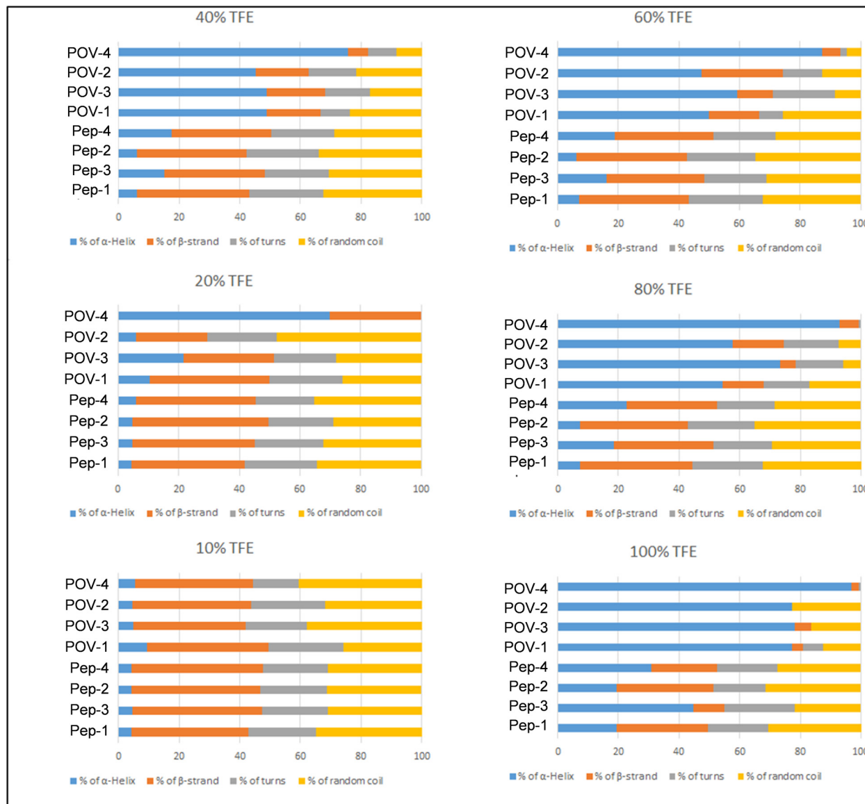
Fig. 7 Percentage of \alpha -helix (blue), \beta -strand (orange), turns (grey) and random coil (yellow) for peptides and POV-hybrids in 10%, 20%, 40%, 60%, 80% and 100% TFE solution.
