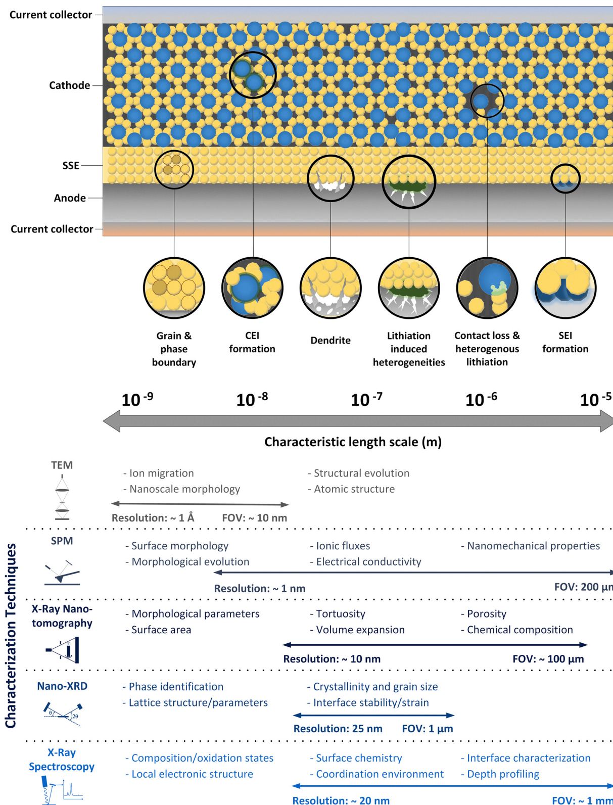
Fig. 1 Overview of interfacial degradation phenomena in solid-state batteries along with their approximate characteristic length scales and the most relevant micro- and nanoscale characterization techniques. Each technique is detailed with its specific applications and properties it can assess in solid-state battery research, along with information about its resolution and typical high-resolution field of view. References for the individual techniques are provided in Table S1 in the SI.
