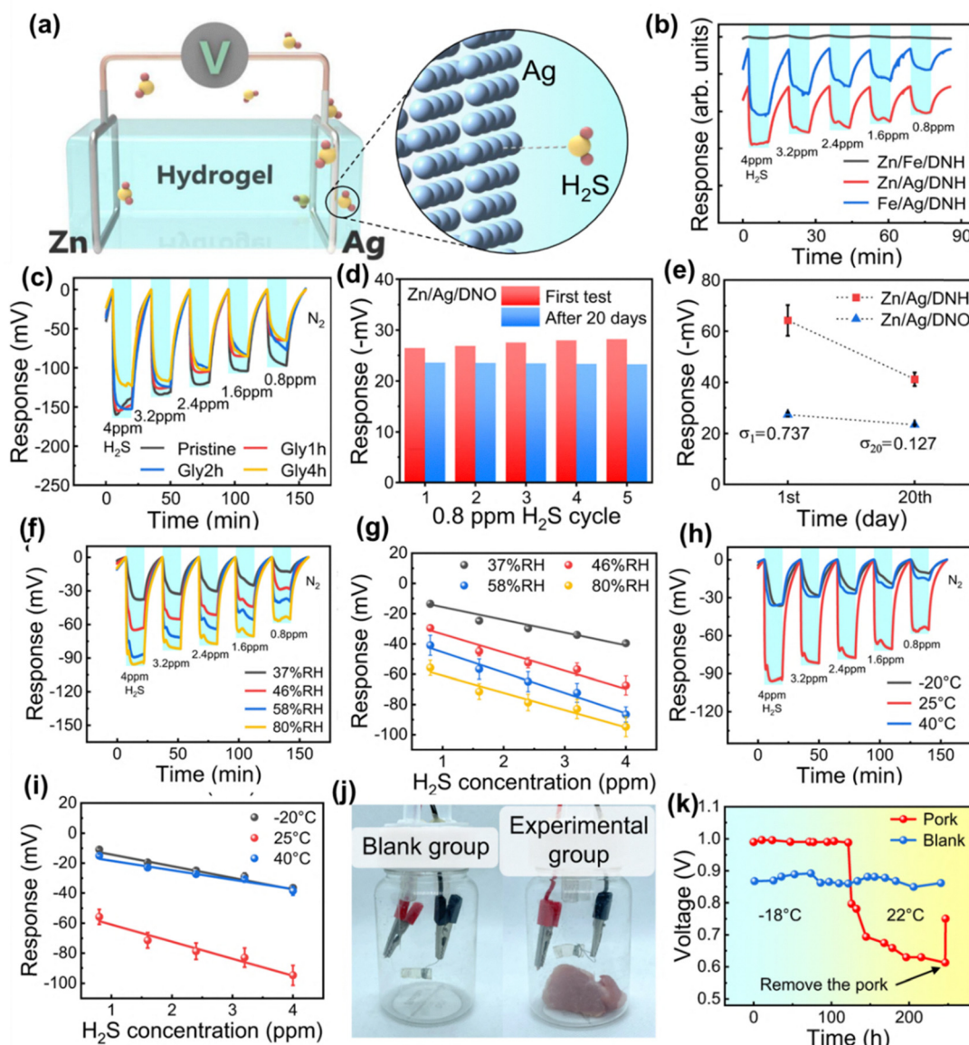
Fig. 13 (a) Schematic illustration of the self-powered H 2 S sensor based on Zn/Ag electrodes and a hydrogel electrolyte. (b) Comparison of H 2 S sensing responses for different electrode configurations (Zn/Ag, Zn/Fe, and Fe/Ag). (c) Dynamic response of the sensor to various H 2 S concentrations (0.8–4 ppm) with different hydrogel modifications. (d) Long-term stability test showing sensor response over 20 days with repeated H 2 S exposure cycles. (e) Signal degradation analysis of Zn/Ag and Zn/Fe electrodes over time under continuous H 2 S exposure. (f) Humidity-dependent response of the sensor across different relative humidity (RH) levels. (g) Sensitivity comparison of the sensor under varying humidity conditions (37–80% RH). (h) Temperature-dependent H 2 S sensing response at –20 °C, 25 °C, and 40 °C. (i) Effect of temperature variations on sensor response across different H 2 S concentrations. (j) Application of the sensor in food spoilage detection, comparing a blank group with pork samples. (k) Real-time voltage response of the sensor during food spoilage monitoring, showing H 2 S accumulation over time. Reproduced with permission, 60 Creative Commons Attribution 4.0 International License Copyright © 2023 Springer Nature.
