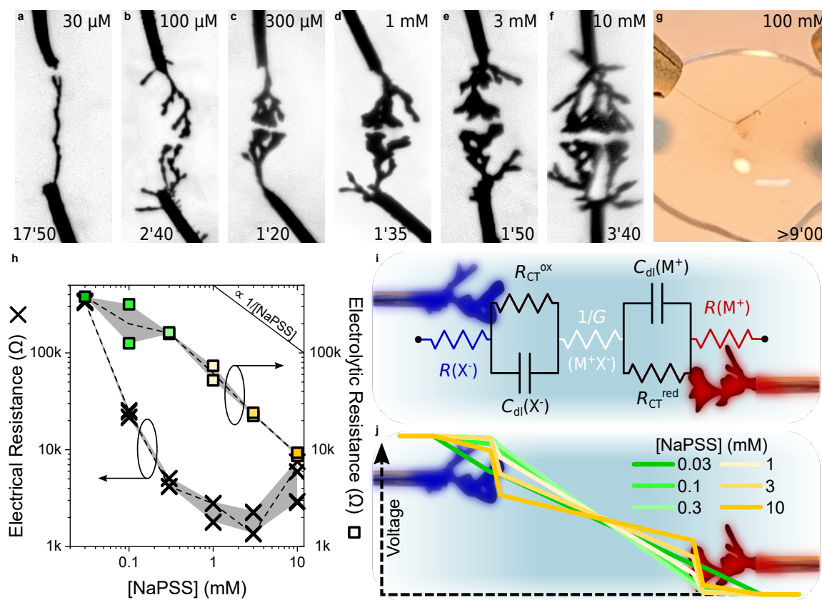
Figure 2: Influence of the Concentration of NaPSS on CPD Morphogenesis in Water | a-f , Optical pictures of CPD growths ( 4 \text{ V}_p , 0 \text{ V}_{off} , 80 \text{ Hz} , 50\%_{dc} , 10 \text{ mM} EDOT and 10 \text{ mM} BQ) in aqueous media with different NaPSS concentrations (values displayed at the top of each picture). Each image was taken a few seconds before CPDs merged (applied-voltage duration displayed at the bottom of each picture). g , Photograph of the electrochemical setup under the same experimental conditions as previously described, but with 100 \text{ mM} of NaPSS. Despite the absence of CPD between the wires, the presence of an electrogenerated material is visible. h , Dependence of the electrical resistance (through each CPD displayed in Fig. 3.a-f after they merged) and the electrolytic resistance (evaluated by impedancemetry at 10 \text{ kHz} with a silver wire) on the concentration of NaPSS in the growth media. i , 7-Element equivalent circuit highlighting the contribution of [NaPSS] on the ohmic resistance of the medium and the CPDs as both an electrolyte and a doping counter-ion carrier. j , Simulated voltage drop according to the equivalent circuit presented in Fig. 3.i, with R_{CT}^{ox} = R_{CT}^{red} = 10 \text{ k}\Omega , R(X^-) = R(M^+) defined as half the experimental value of the CPD electrical resistance once merged and 1/G as the experimental value of the electrolytic resistance measured with a silver wire. Blue indicates the point of highest potential in the circuit, whereas red indicates the point of lowest potential.
