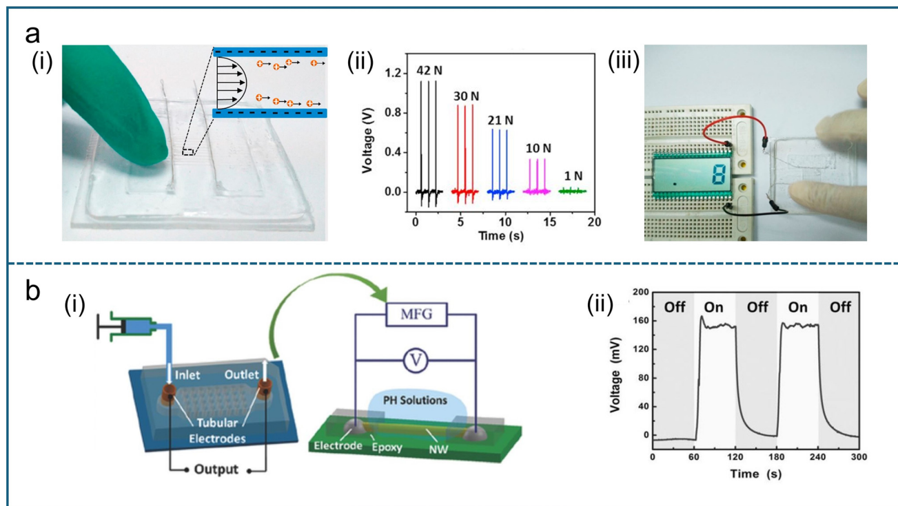
Fig. 25 Applications of a microfluidic energy generator. a) (i) Schematic of a flexible MFNG which consists of ten microchannels. The width of each channel is 100\ \mu\text{m} . a) (ii) The voltage generated by the MFNG at different external forces. a) (iii) Photo of the LCD powered by the MFNG directly. Reproduced with permission. 375 Copyright 2016, Elsevier. b) (i) Schematic of the microfluidic nanogenerator with a porous patterned structure in the microchannel, where the microfluidic nanogenerator supplied energy to a single NW based pH sensor. b) (ii) Voltage generated from the microfluidic when a 1\ \mu\text{M} KCl solution flows through the device at 0.4\ \text{mL min}^{-1} . Reproduced with permission. 31 Copyright 2015, Wiley.
