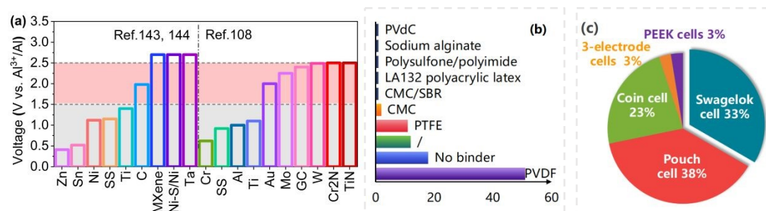
Figure 16. a) The oxidative stability, in terms of the voltage versus Al/Al^{3+} , of Ni-S/ Ni^{143} , MXene and other various current collector materials 144 in AlCl_3/[EMIm]Cl electrolyte with molar ratios of 1.3 (left) and 2.0 (right). Adapted from Wang, S. et al., Adv Sci (Weinh) 108 . Licensed under CC BY 4.0. ©2018 Wiley. b) Number of publications reporting various binders used in AGDIBs based on literature survey ('/' indicates not mentioned). c) Cell configurations applied in AGDIBs from the literature survey.
