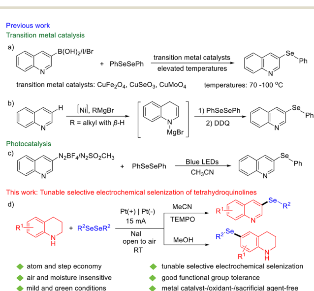
Fig. 2 Synthesis of C-3 selenylated quinolines.
