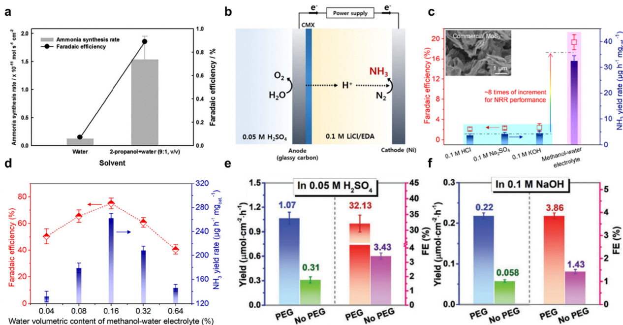
Fig. 6 Solvent effect. (a) Effect of electrolyte medium of water or 2-propanol on NH 3 synthesis rate and FE. Reproduced with permission. 65 Copyright 2016, The Electrochemical Society. (b) Schematic for ethylenediamine (EDA)-based NH 3 synthesis. Reproduced with permission. 64 Copyright 2016, The Electrochemical Society. (c) Comparison of NRR performance achieved by commercial MoS 2 in aqueous electrolytes and methanol–water electrolyte. The inset is the scanning electron micrograph image of used commercial MoS 2 . (d) NRR FE and NH 3 yield rate over FeOOH/CNTs at the applied potential of -1.2 V vs. Ag/AgCl for 2 h in methanol–water electrolytes with water volumetric content of 0.04, 0.08, 0.16, 0.32, and 0.64%, respectively. Reproduced with permission. 66 Copyright 2021, American Chemical Society. NH 3 yield and FE of TiO 2 nanoarray electrode in (e) 0.05 M H 2 SO 4 , and (f) 0.1 M NaOH electrolyte with/without 20 wt% poly(ethylene glycol) PEG400. Reproduced with permission. 82 Copyright 2021, Wiley-VCH.
