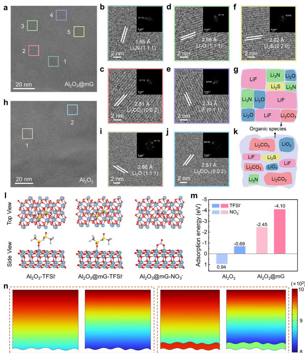
Fig. 5 Compositional analysis and mechanistic investigation of SEI. (a) Cryo-TEM images of the SEI formed by \text{Al}_2\text{O}_3@\text{mG} . (b)–(f) Representative HRTEM images showing (b) \text{Li}_3\text{N} , (c) \text{Li}_2\text{CO}_3 , (d) \text{Li}_2\text{O} , (e) \text{LiF} , and (f) \text{Li}_2\text{S} phases from region 1–5. (g) Schematic of the SEI formed by \text{Al}_2\text{O}_3@\text{mG} . (h) Cryo-TEM images of the SEI formed by \text{Al}_2\text{O}_3 . (i) and (j) Representative HRTEM images of (i) \text{Li}_2\text{O} and (j) \text{Li}_2\text{CO}_3 phases from region 1, 2. (k) Schematic of the SEI formed by \text{Al}_2\text{O}_3 . (l) Adsorption structures of \text{TFSI}^- and \text{NO}_3^- on \text{Al}_2\text{O}_3 and \text{Al}_2\text{O}_3@\text{mG} . (m) Corresponding adsorption energies. (n) Finite element method simulations of the spatial \text{Li}^+ distributions of \text{Al}_2\text{O}_3 (left panels) and \text{Al}_2\text{O}_3@\text{mG} (right panels).
