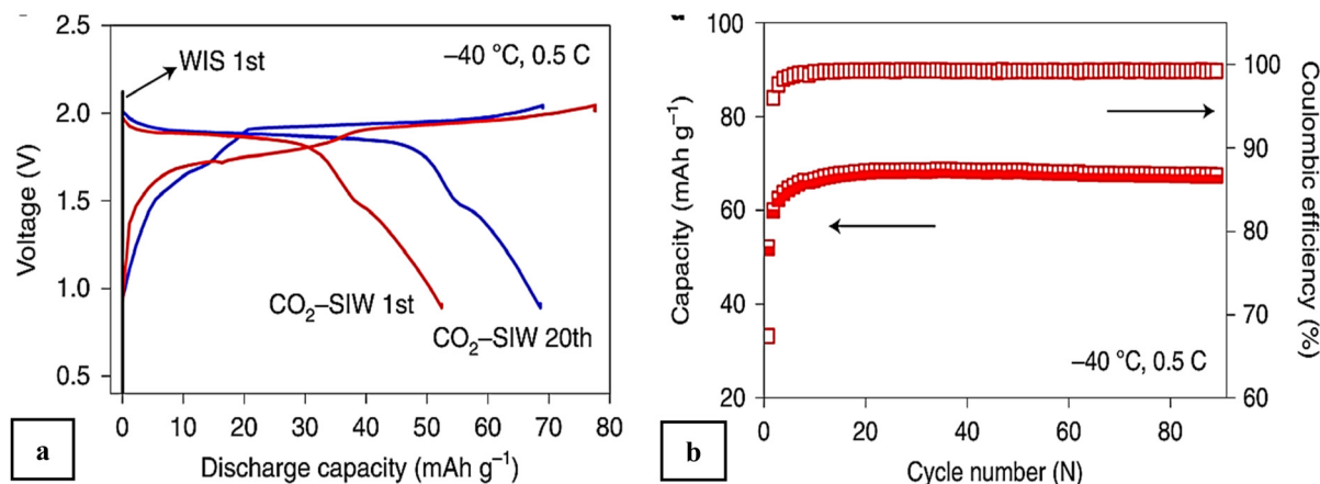
Fig. 14 (a) Initial charge/discharge profiles of a \text{Mo}_6\text{S}_8/\text{LMO} aqueous full cell using \text{CO}_2\text{-SIW} and \text{WIS} electrolytes. (b) Cycling stability of the \text{Mo}_6\text{S}_8/\text{LMO} aqueous full cell with \text{CO}_2\text{-SIW} electrolyte at -40^\circ\text{C} and 0.5\text{C} . Reproduced with permission from ref. 225.
