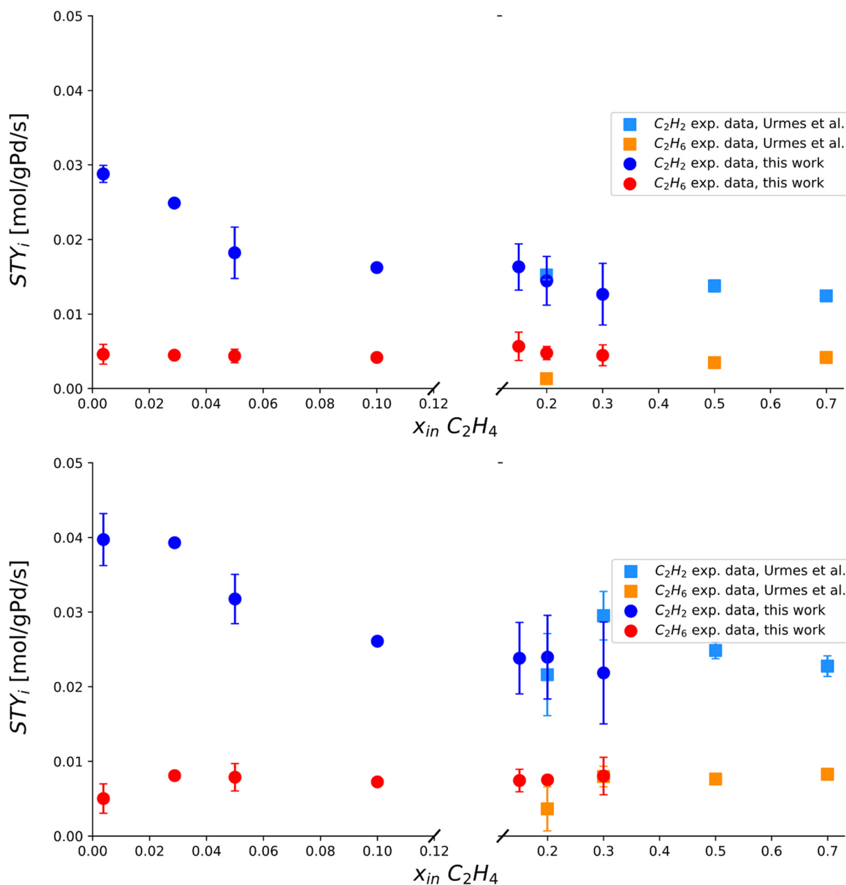
Fig. 4 Experimentally measured space-time yields of C_2H_2 and C_2H_6 ( STY_{C_2H_2} [ \text{mol gPd}^{-1} \text{s}^{-1} ] and STY_{C_2H_6} [ \text{mol gPd}^{-1} \text{s}^{-1} ]) plotted against the inlet molar fraction of C_2H_4 . Top) Trend obtained at 323 K, i.e. 50 °C. Bottom) Trends obtained at 333 K, i.e. 60 °C. The x -axis is reported with a broken plot representation to precisely quantify the behavior across the composition range investigated. Includes experimental data by Urmès et al. and experimental data from this work. The standard deviation of experimental measurements is reported through error bars for points whose reproducibility has been verified through at least two repeated experiments.
