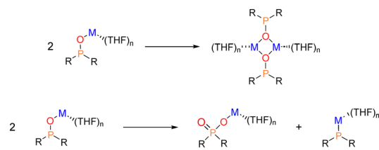
Scheme 7 Deactivation processes of alkali metal diorganylphosphinites M-OPR 2 : dimerization (top) and dismutation (bottom).
