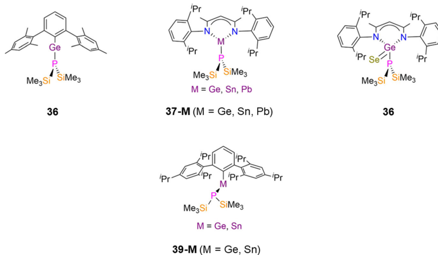
Fig. 10 Mononuclear group 14 P'' complexes [Ge(P'')(Ar^{Mes})] ( Ar^{Mes} = C_6H_3Mes_{2-2,6} ) ( 36 ), [M(DippPnacac)(P'')] ( 37-M ; M = Ge, Sn, Pb, DippPnacac = CH\{(CH_3)_2CN(Dipp)\}_2 ; Dipp = C_6H_3^iPr_2-2,6 ), [Ge(Se)(DippPnacac)(P'')] ( 38 ), [M(Ph^*)(P'')] ( 39-M ; M = Ge, Sn, Ph^* = C_6H_3Trip-2,6 , Trip = C_6H_2^iPr_3-2,4,6 ).
