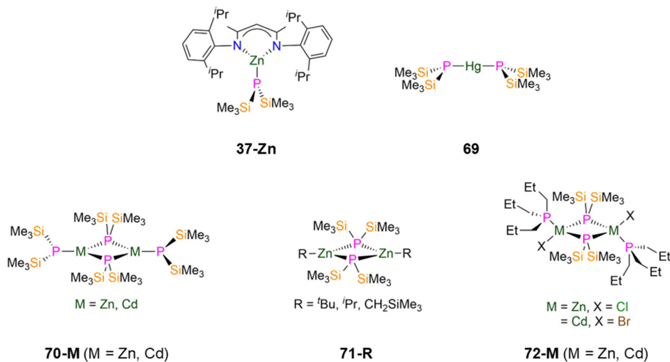
Fig. 20 Monomeric and dimeric group 12 P'' complexes [Zn(\text{DippNacnac})(P'')] ( 37-Zn ; DippNacnac = \text{CH}\{(\text{CH}_3)_2\text{CN}(\text{Dipp})\}_2 ; Dipp = \text{C}_6\text{H}_3\text{Pr}_2\text{-2,6} ), [\text{Hg}(P'')]_2 ( 69 ), [M(P'')(\mu\text{-}P'')]_2 ( 70-M , M = Zn, Cd), [Zn(R)(\mu\text{-}P'')]_2 ( 71-R , R = ^t\text{Bu} , ^i\text{Pr} , \text{CH}_2\text{SiMe}_3 ), [M(P''\text{Pr}_3)(X)(\mu\text{-}P'')]_2 ( 72-Zn : M = Zn, X = Cl; 72-Cd : M = Cd, X = Br).
