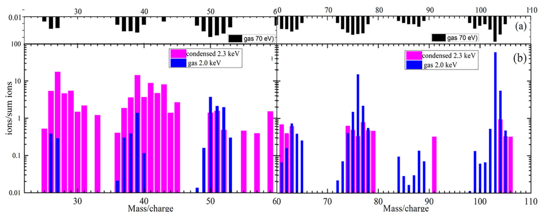
Fig. 8 Yields of cations with mass/charge from m/z = 20 – 110 produced in the gas phase and desorbed in the condensed phase (multilayer film) indicated in blue and magenta, respectively. At the top, to better highlight the differences, yields of cations formed in the gas phase by 70 eV electrons are included.
