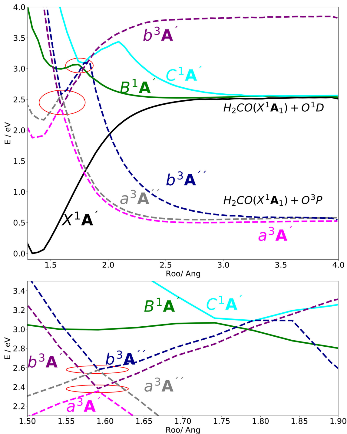
Fig. 19 (Upper) the adiabatic PE curves along the \text{OO} stretching mode for the X^1A' , B^1A' , C^1A' , a^3A' , b^3A' , a^3A'' and b^3A'' states. (Lower) the adiabatic PE curves along \text{O-O} stretching mode, zooming in geometries in the range 1.55 < R_{\text{OO}} < 1.80 (indicated by red circles in the upper panel). The bonding angle \theta_{\text{COO}} and the stretching mode R_{\text{CO}} are fixed at the equilibrium structure values 117.905^\circ and 1.27 , respectively.
