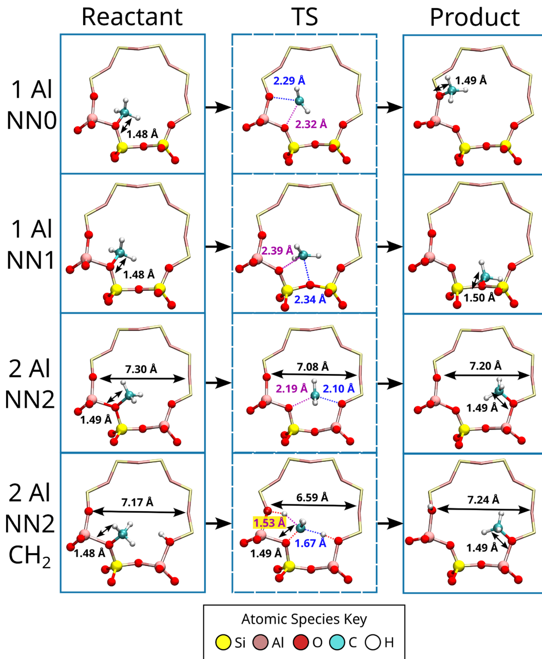
Fig. 6 Migration of SMS on H-SSZ-13 from the \text{-O-Al-O-} site in the 8-MR to: the same T-site (NN0); a T-site one nearest neighbour (NN1) site away; and a T-site two nearest neighbour (NN2) sites away, as labelled. The H-SSZ-13 framework with isolated (1Al) and paired (2Al) Al substituted T-sites are represented in the top and bottom two rows, respectively. The reaction denoted as 2Al NN2 \text{CH}_2 proceeds through a carbene-like intermediate. The activation energies for the corresponding reactions are shown in Table 2.
