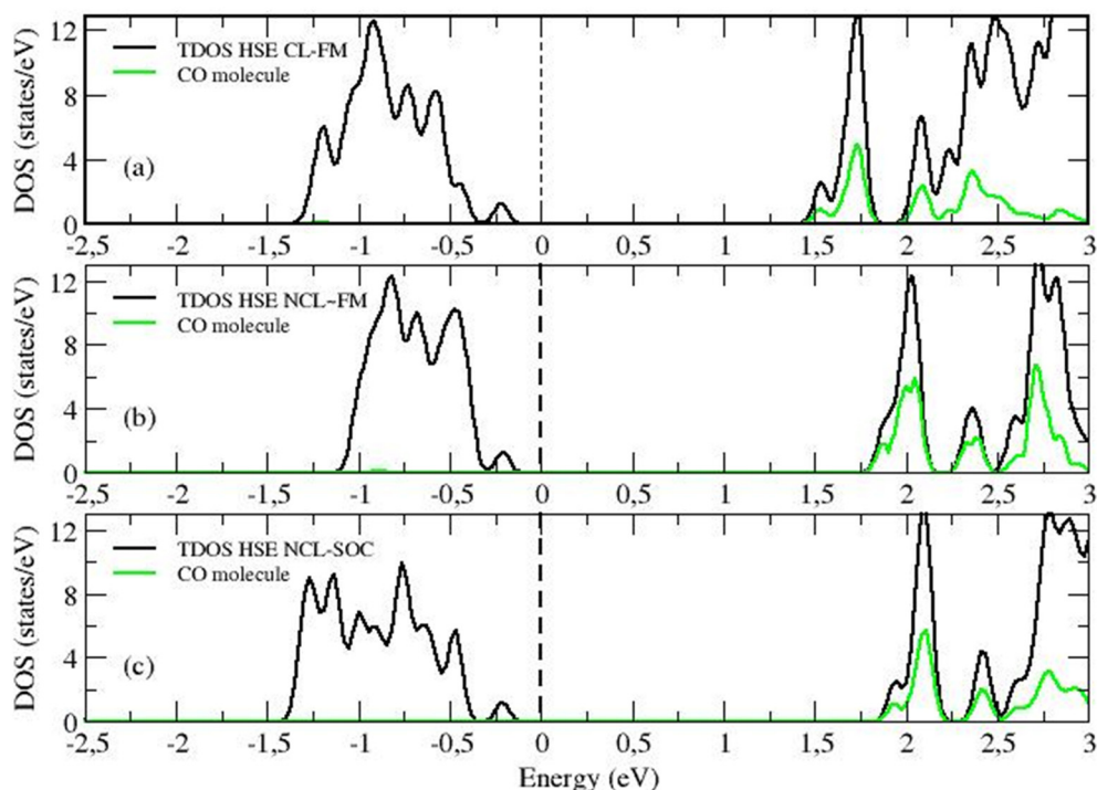
Fig. 8 The total density of state (TDOS, black line) of the CO adsorbed-UO 2 (111) system as computed by HSE06 together with the projected density of state on the molecular CO orbitals (green). (a) Collinear FM (HSE CL-FM) case, (b) non-collinear nearly FM (HSE NCL ~ FM) case, and (c) non-collinear with spin–orbit coupling (HSE NCL-SOC) case.
