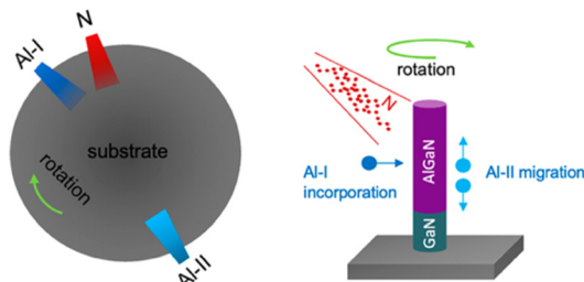
Fig. 6 Illustration of different Al adatom kinetics at the growth front when Al sources in two different locations are used. 89
