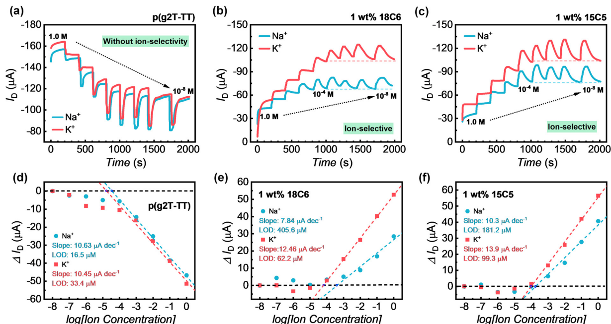
Fig. 4 Real-time cation detection using the studied OECTs and the response of the Na + and K + OECTs to a change in the electrolyte concentration (NaCl, blue; and KCl, red) from 1 M to 10^{-8} M ( V_D = -0.6 V): (a) p(g2T-TT) at V_G = -0.6 V, (b) 1 wt% 18C6-mixed p(g2T-TT) at V_G = -0.5 V, and (c) 1 wt% 15C5-mixed p(g2T-TT) at V_G = -0.8 V. Calibration curves of the measured current at equilibrium to NaCl and KCl aqueous solutions with different concentrations: (d) p(g2T-TT), (e) 1 wt% 18C6-mixed p(g2T-TT), and (f) 1 wt% 15C5-mixed p(g2T-TT).
